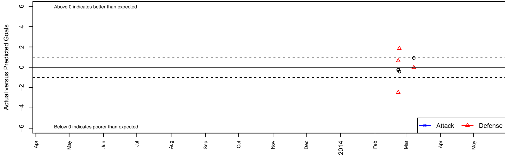
IUSC Brasil B01 Dots are actual minus expected GF (blue circles) and GA (red triangles). Blue line is smoothed change in attack strength. Red is smoothed change in defense strength.
